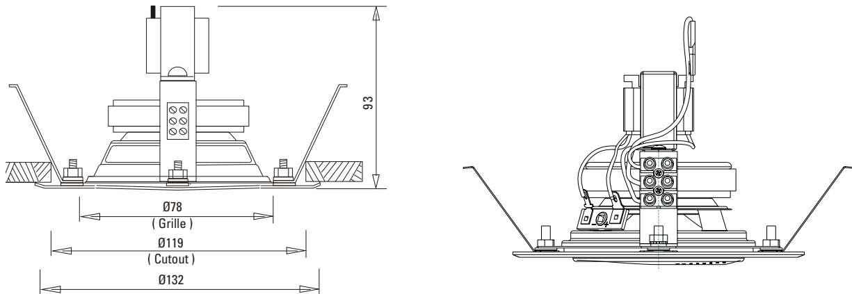
Side view (unit: mm)
